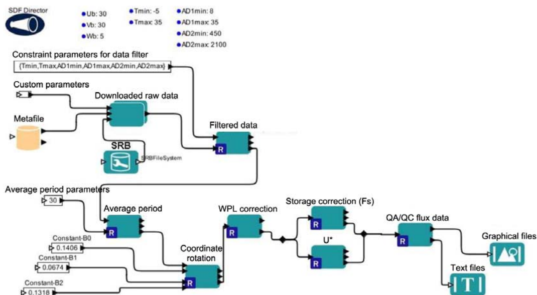
Figure 2. Workflow constructed in Kepler system
